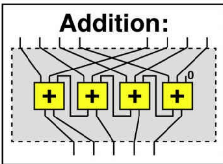
Figure 2.7: Any well-defined computation can be performed by cleverly combining nothing but NAND gates. For example, the addition and multiplication modules above both input two binary numbers represented by 4 bits, and output a binary number represented by 5 bits and 8 bits, respectively. The smaller modules NOT, AND, XOR and + (which sums three separate bits into a 2-bit binary number) are in turn built out of NAND gates. Fully understanding this figure is extremely challenging and totally unnecessary for following the rest of this book; I'm including it here just to illustrate the idea of universality—and to satisfy my inner geek.
