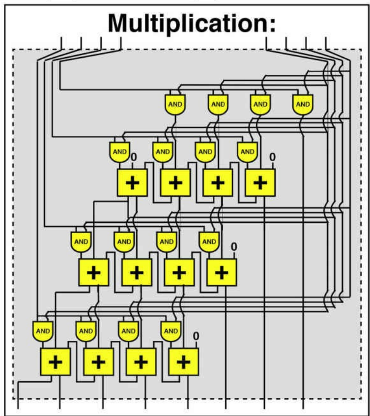
Figure 2.7: Any well-defined computation can be performed by cleverly combining nothing but NAND gates. For example, the addition and multiplication modules above both input two binary numbers represented by 4 bits, and output a binary number represented by 5 bits and 8 bits, respectively. The smaller modules NOT, AND, XOR and + (which sums three separate bits into a 2-bit binary number) are in turn built out of NAND gates. Fully understanding this figure is extremely challenging and totally unnecessary for following the rest of this book; I'm including it here just to illustrate the idea of universality—and to satisfy my inner geek.
