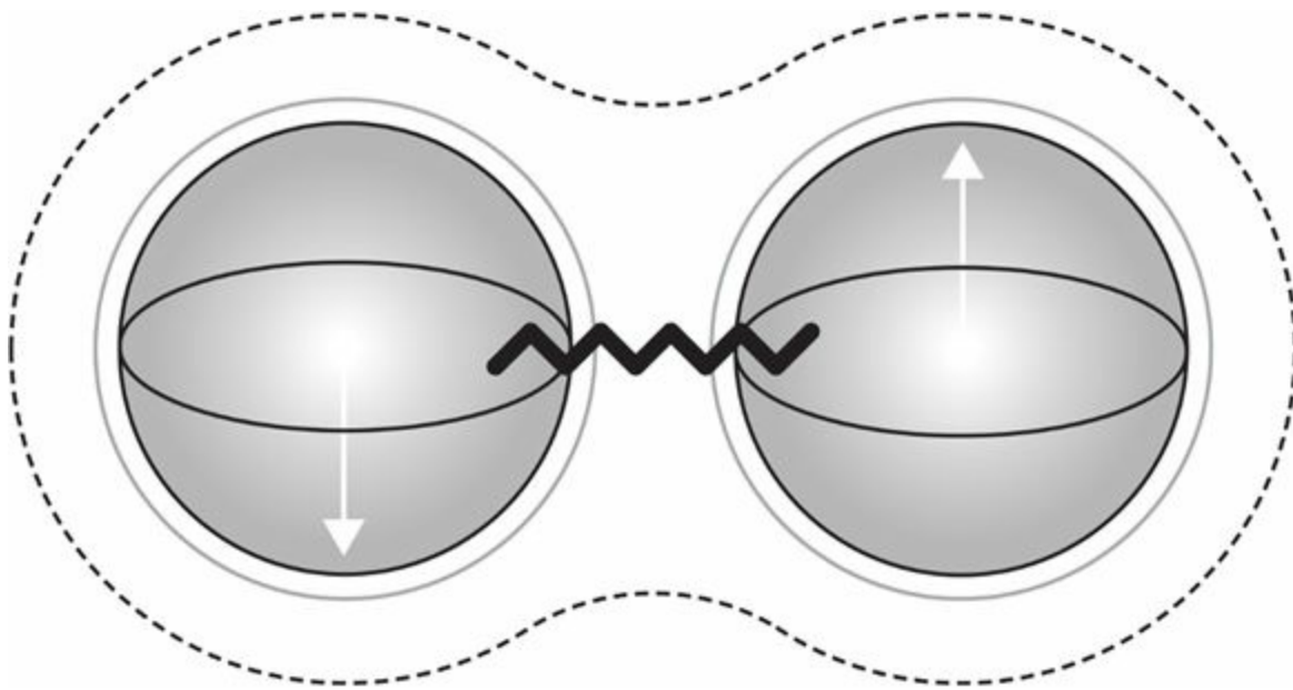
FIGURE 1-3: Entangled qubits influence each other.
