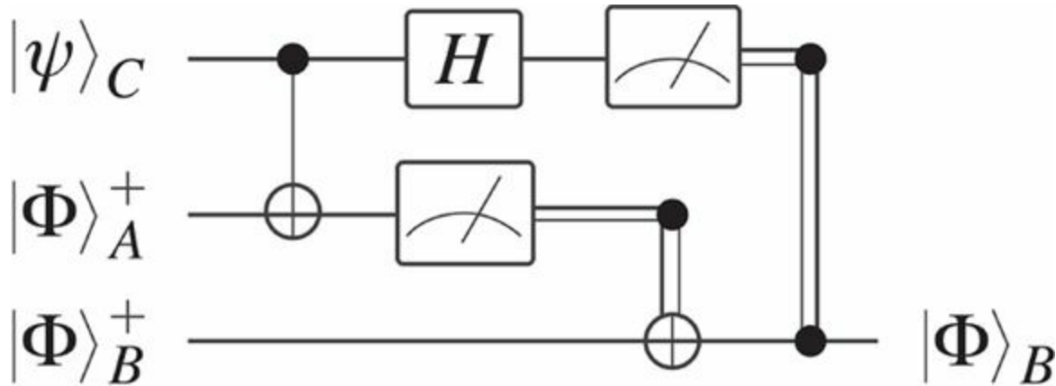
FIGURE 12-3: An example of a quantum circuit.
