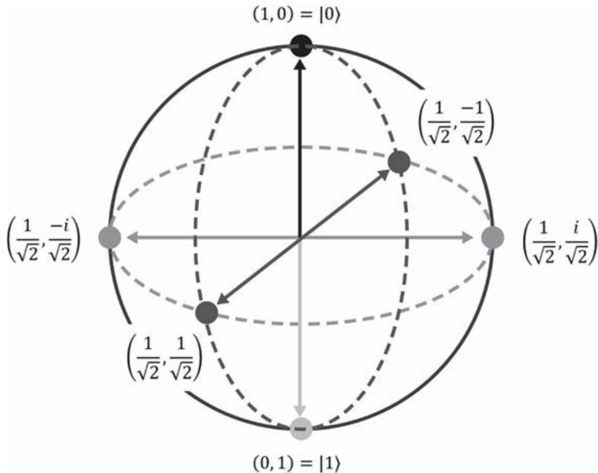
FIGURE 12-1: A Bloch sphere.
