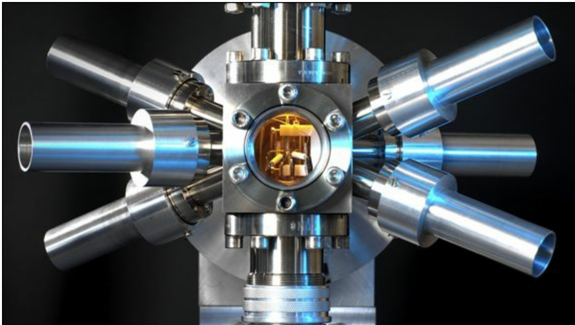
FIGURE 4-4: A strontium ion optical clock.
