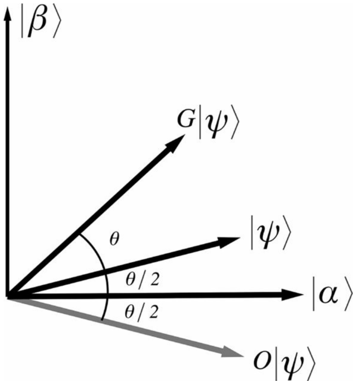
FIGURE 5-6: Grover's algorithm finds needles in haystacks faster.
